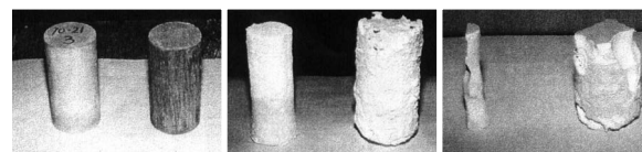
"An Enhancement in the Nature of Concrete with a Multiplicative Cement Crystal-Type Concrete Material", Central Research Laboratory of Nikki Shoji in association with Hosei University, Japan
